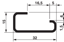
Dimensional drawing
